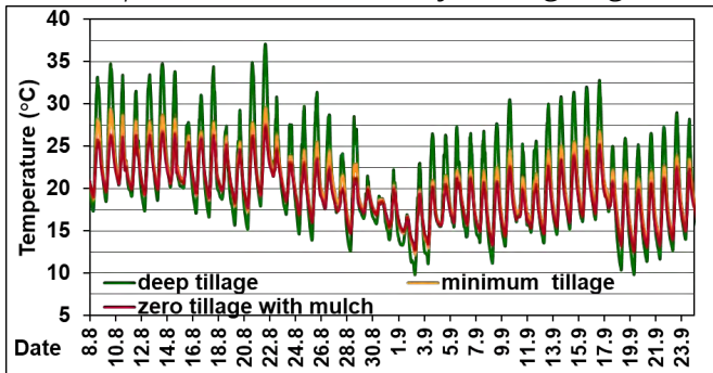
Soil temperature and humidity during August and September under different tillage practices
