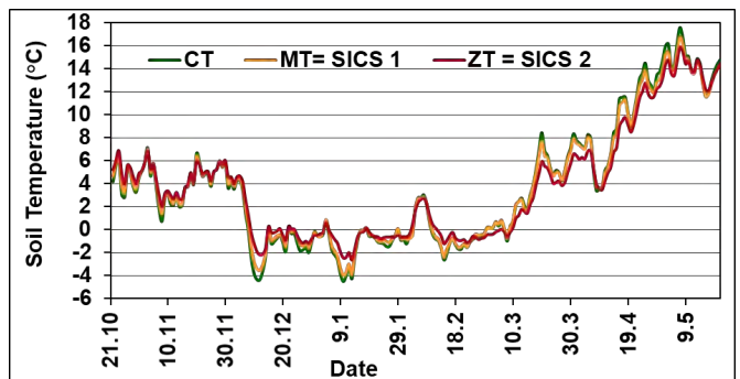
Soil temperature (5 cm depth) under different tillage during winter wheat vegetation
