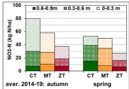
Nitrate nitrogen content in soil profile before and after winter
